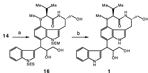
Scheme 8. Reagents and conditions. (a) \text{OsO}_4 , TMEDA, \text{CH}_2\text{Cl}_2 -90^\circ\text{C} . (b) TBAF, neat at 0.1 mm Hg.
