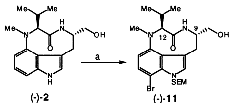
Scheme 5. Reagents and conditions. (a) 1. TBS-Cl, imidazole, DMF, rt; 2. SEM-Cl, NaH, THF, -15^{\circ}\text{C} ; 3. NBS, DMF, -15^{\circ}\text{C} ; 4. TBAF, THF, rt.
