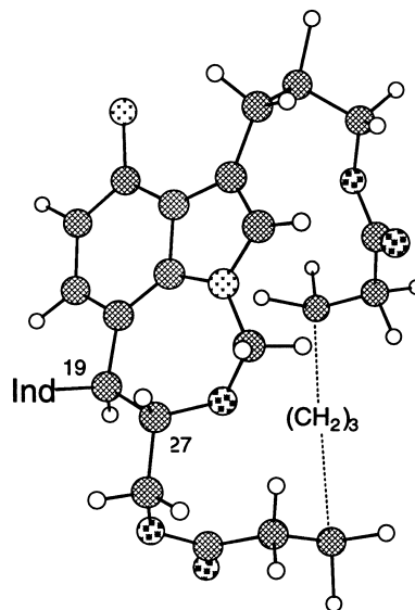
Figure 5. A partial stereoview of the lactam 21 . ⊗, ⊙, ⊕, ○, represent C, N, O, and H, respectively.
