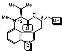
(–)-indolactam V ( 2 )
