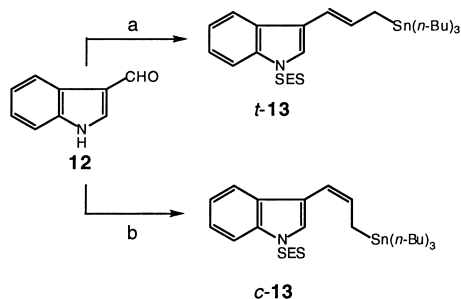
Scheme 6. Reagents and conditions. (a) 1. SES-Cl, NaOH, cetyltrimethylammonium chloride, \text{CH}_2\text{Cl}_2 , 0^{\circ}\text{C} ; 2. \text{CH}_2=\text{CHMgBr} , THF, -78^{\circ}\text{C} ; 3. \text{Ac}_2\text{O} , Py, rt; 4. n\text{-Bu}_3\text{Sn-Cu}(n\text{-Bu})(\text{CN})\text{Li}_2 , THF, -78^{\circ}\text{C} . (b) 1. same as (a) 1; 2. n\text{-Bu}_3\text{SnCH}_2\text{CH}=\text{PPh}_3 , THF, -78^{\circ}\text{C} \rightarrow \text{rt} .
