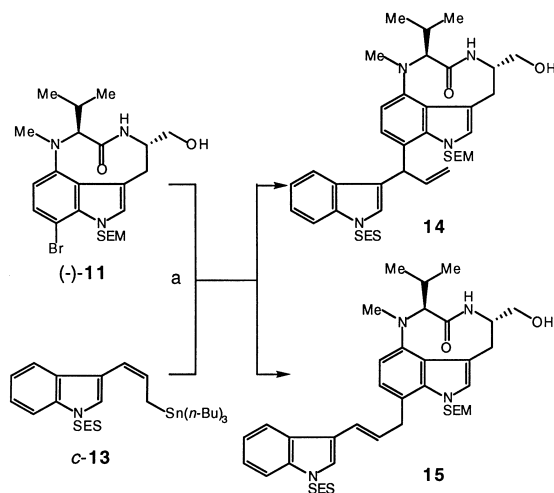
Scheme 7. Reagents and conditions. (a) \text{Pd}(\text{PPh}_3)_4 , TBAI, PhH, 80^{\circ}\text{C} .
