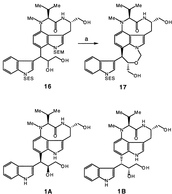
Scheme 9. Reagents and conditions. (a) LiBF 4 (MeCN), CSA, THF, rt.
