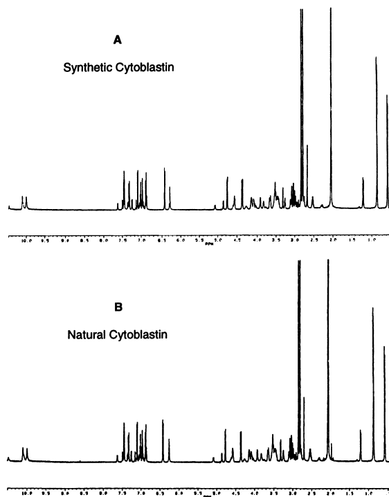
Figure 3. ^1\text{H} NMR spectra (5000 MHz) of the synthetic (Panel A) and natural (Panel B) cycloblastin ( 1 ) in acetone- d_6 .
