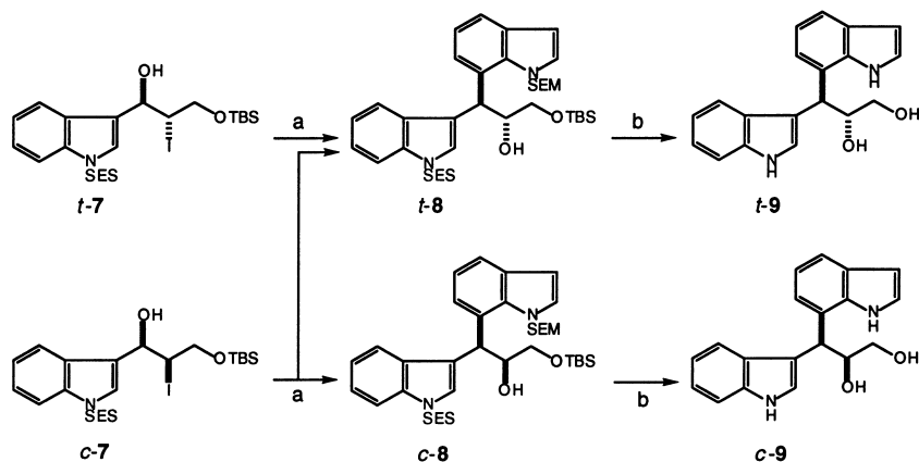
Scheme 3. Reagents and conditions. (a) KHMDS, THF, -78^{\circ}\text{C} , followed by addition of Ce reagent (prepared from N -SEM-7-bromoindole by treatment with n -BuLi, THF, -78^{\circ}\text{C} , \text{ZnCl}_2 , -78^{\circ}\text{C} \rightarrow \text{rt} , then \text{CeCl}_3 , rt), -78^{\circ}\text{C} \rightarrow \text{rt} . (b) TBAF, EDA, DMF, 70^{\circ}\text{C} .
