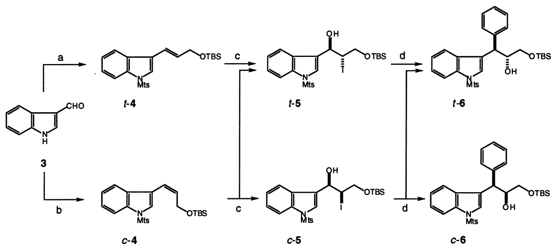
Scheme 2. Reagents and conditions. (a) 1. Mts-Cl, NaOH, Cetyltrimethylammonium chloride, CH 2 Cl 2 , 0 °C; 2. Ph 3 P=CHCO 2 Et, CH 2 Cl 2 , rt; 3. DIBAL, THF, -78 °C; 4. TBS-Cl, imidazole, DMF, rt. (b) 1. same as (a) 1; 2. (CF 3 CH 2 O) 2 P(O)CH 2 CO 2 Me, 9 KHMDS, 18-Crown-6, THF, -78 °C; 3. same as (a) 3; 4. same as (a) 4. (c) I 2 , Ag 2 O, aq THF. (d) KHMDS, THF, -78 °C, followed by addition of PhMgBr, -78 °C→rt.
