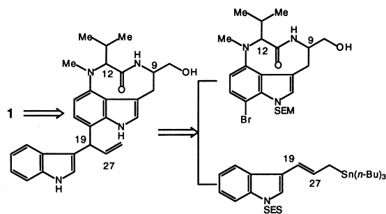
Scheme 4. The second retrosynthetic analysis of cytoblastin ( 1 ).
