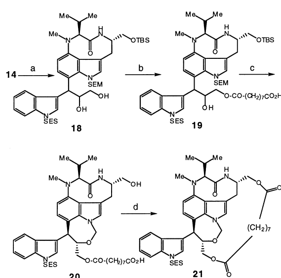
Scheme 10. Reagents and conditions. (a) 1. TBS-Cl, imidazole, DMF, rt. 2. OsO 4 , TMEDA, CH 2 Cl 2 , -90 °C. (b) Azelaic acid, EDAC, DMAP, DMAP·HCl, CH 2 Cl 2 rt. (c) LiBF 4 (MeCN), CSA, THF, rt. (d) EDAC, DMAP, DMAP·HCl, CH 2 Cl 2 , rt.
