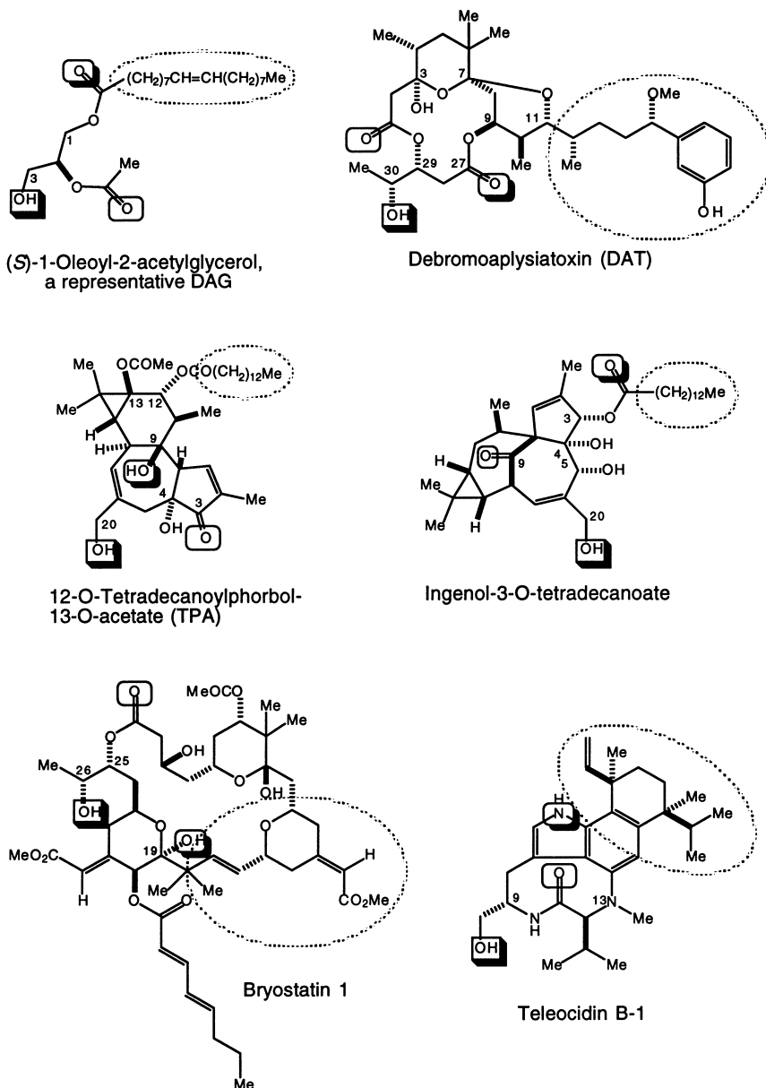
Figure 1. The pharmacophores of various tumor promoters.
