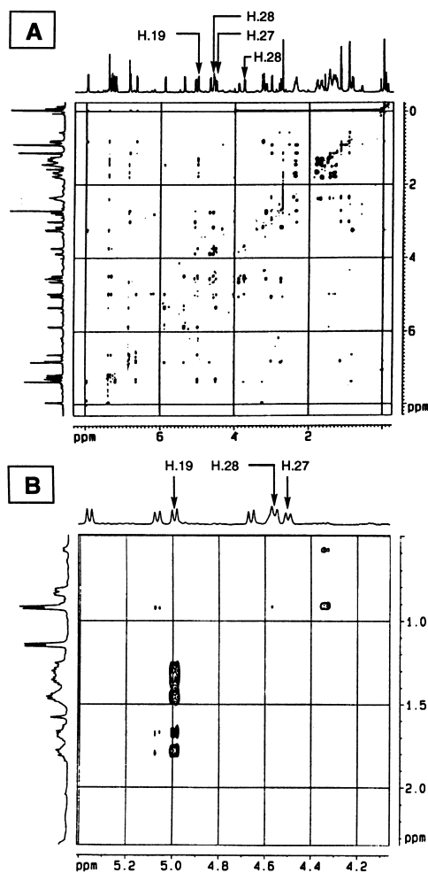
Figure 4. The NOSEY spectrum ( \text{CDCl}_3 ) of 21 . The panel A shows the region of (-0.2-8.2\text{ ppm}) \times (-0.2-8.2\text{ ppm}) , whereas the panel B shows the region of (4.1-5.4\text{ ppm}) \times (0.5-2.3\text{ ppm}) . The chemical shift for the C.19–H, C.27–H, C.28–H, and C.28–H are 4.99 ppm (d), 4.49 (ddd), 4.56 (dd), and 3.73 (dd), respectively.
