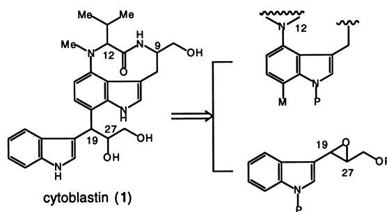
Scheme 1. The first retrosynthetic analysis of cytoblastin ( 1 ).
